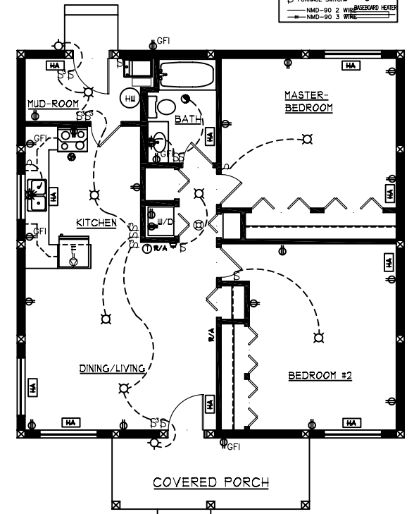
ELECTRICAL PLAN
