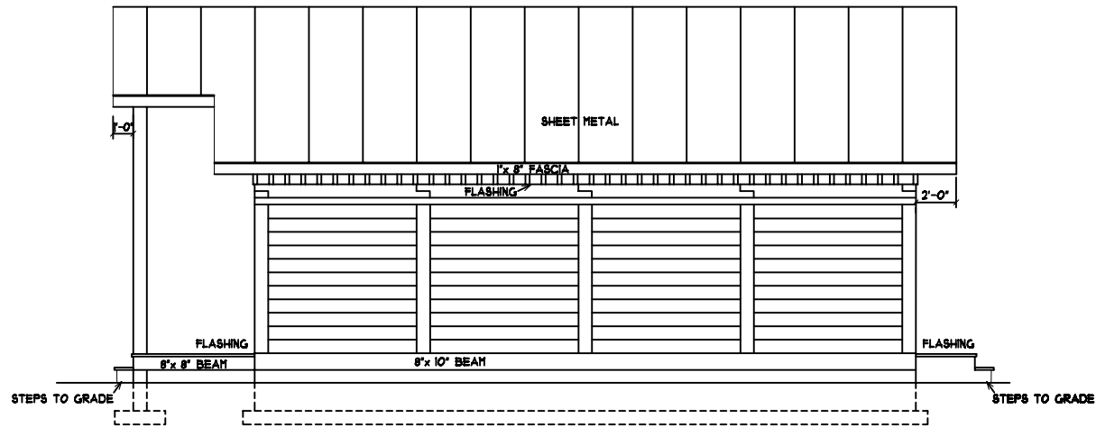
LEFT ELEVATION
