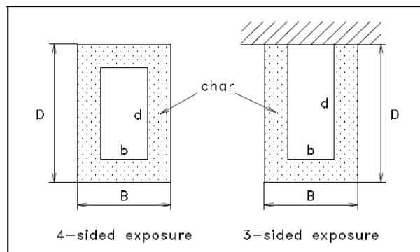
Figure 2 Symbols for cross-sectional dimensions
